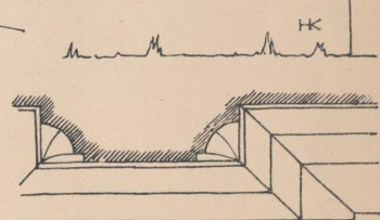
LISENE AM CHOR 1:10
