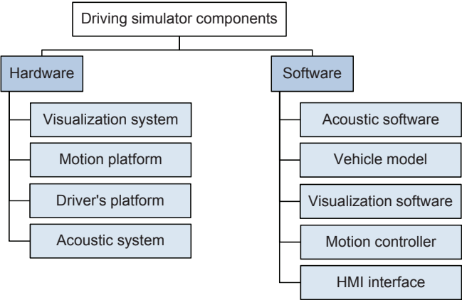
Figure 4-10: The driving simulator components as identified and classified in HASSAN’S method – reconstructed according to Reference [Has14, p. 89]
