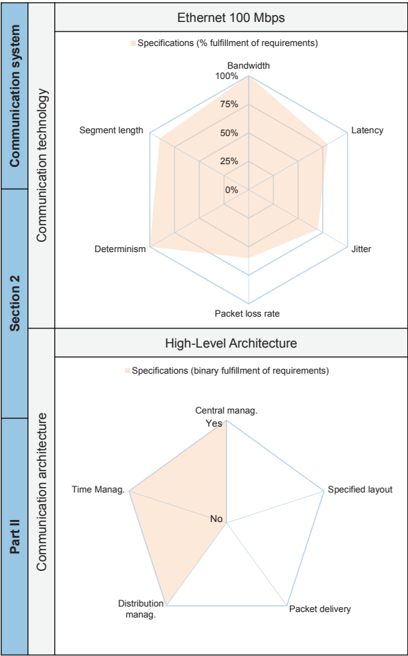
Figure 5-16: Specification/requirement radar charts of the selected communication components
